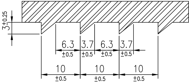
DETAILS OF THREAD SCALE 2 : 1
